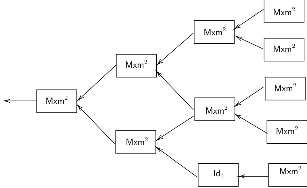
Figure 6.1: Neural network diagram for Mxm^5 .
