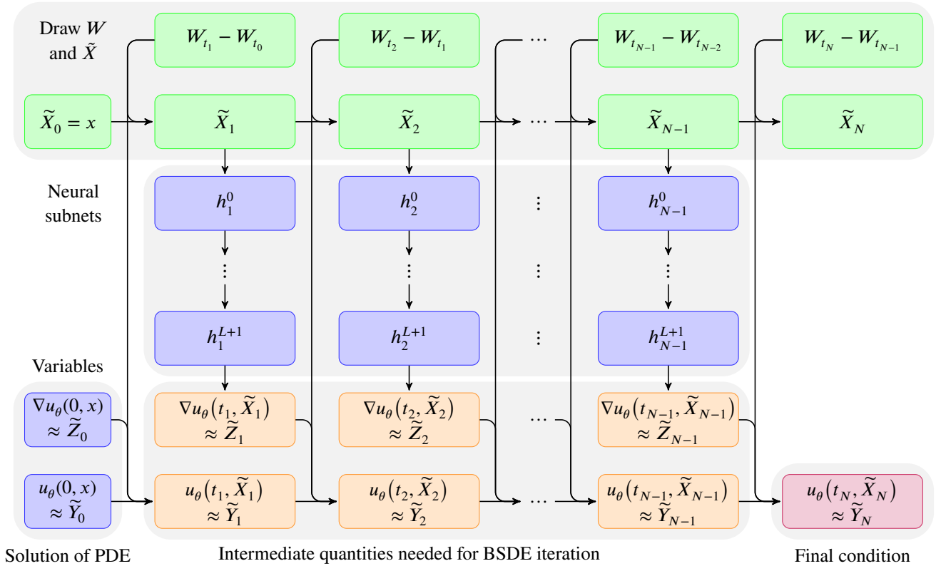
FIGURE 6 Illustration of the complete deep BSDE solver model adapted from [44, 70] in the case \sigma = I_{d \times d} . The two upper rows express the evolution of the forward process \{X_t\}_{t=0}^T starting at \tilde{X}_0 = x (green). The unknown parameters for u_\theta(0, x) and \nabla u_\theta(0, x) (blue, left) as well as the parameters in the neural network approximating \tilde{Z}_n , n = 1, \dots, N-1 (blue, center) are learned by training. The intermediate values \tilde{Y}_n and \tilde{Z}_n , n = 1, \dots, N-1 (orange) are needed to establish the link between the desired PDE solution value u(0, x) \approx \tilde{Y}_0 with the given final value \tilde{Y}_N = g(\tilde{X}_N) (red).
