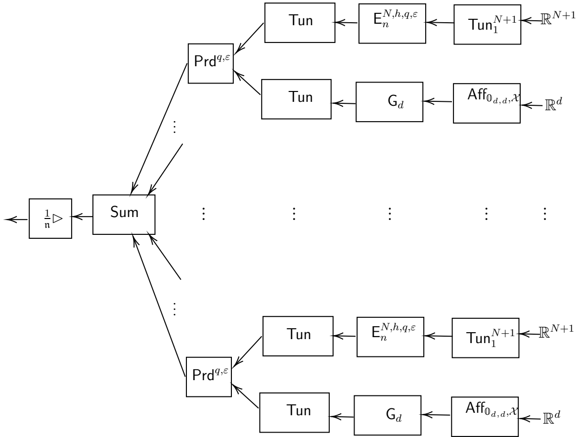
Figure 7.2: Neural network diagram for the UES_{n, G_d, \Omega, n}^{N, h, q, \epsilon} network.
